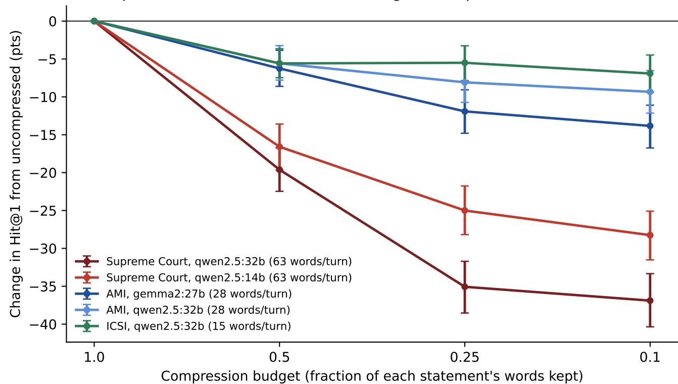
Compression costs six times more on long-turn corpora than short-turn ones
