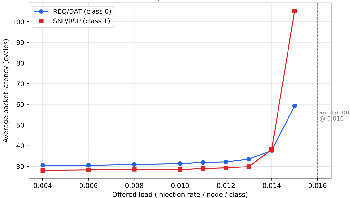
Latency vs. Offered Load
