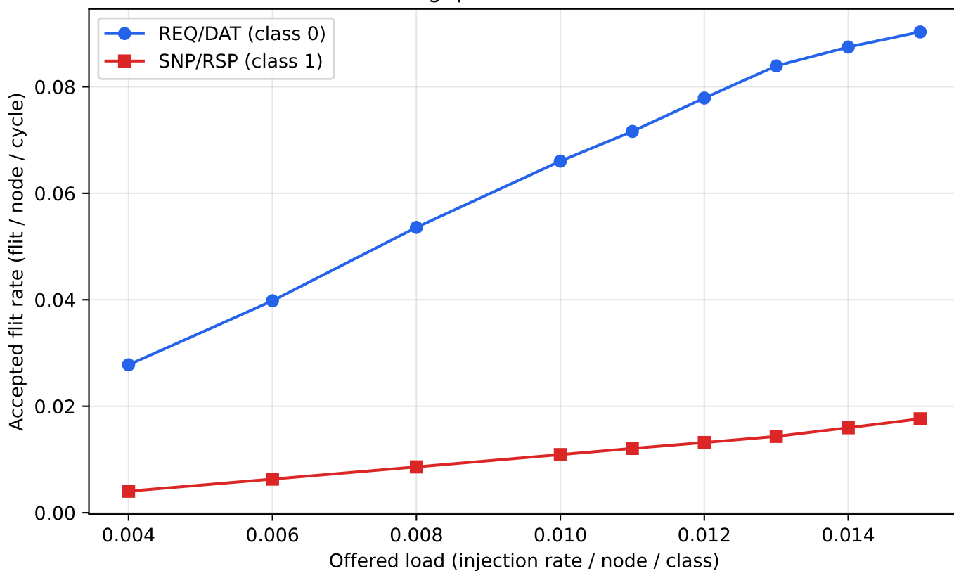
Throughput vs. Offered Load
