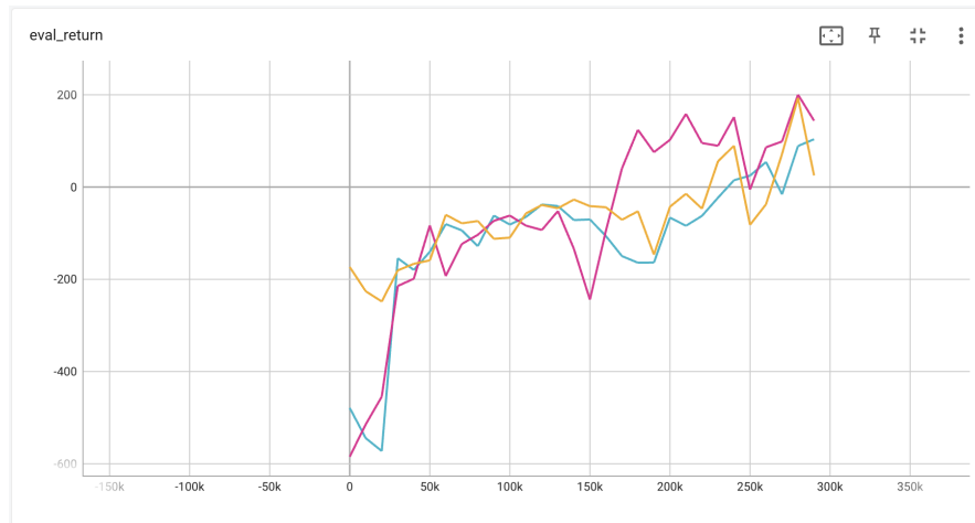
Figure 2: Eval return plot for LunarLander-v2 across 3 seeds
