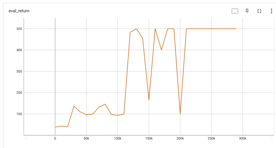
Figure 1: Eval return plot for CartPole-v1
