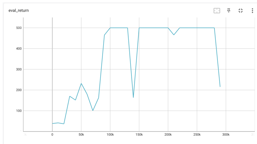
Figure 1: Eval return plot for CartPole-v1
