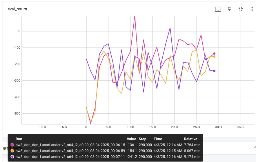
Figure 2: Eval return plot for LunarLander-v2 across 3 seeds
