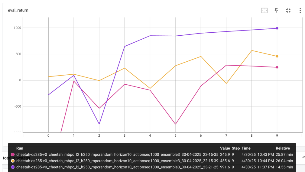
Figure 9: Eval return for Cheetah: baseline (pink), dyna (yellow), mbpo (purple)
