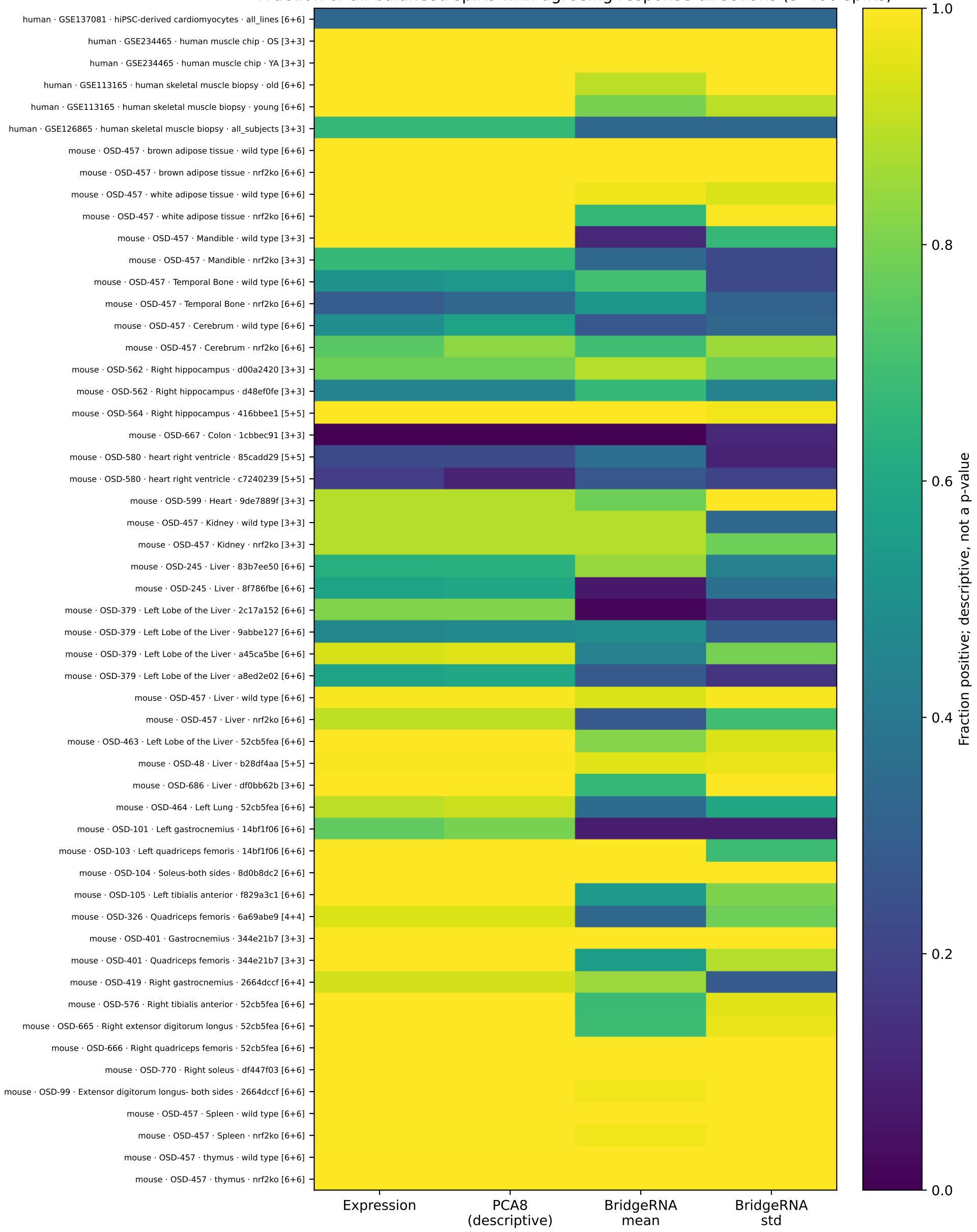
General space-biology survey: directional split-sample stability Fraction of all balanced splits with agreeing response directions (3-400 splits)
