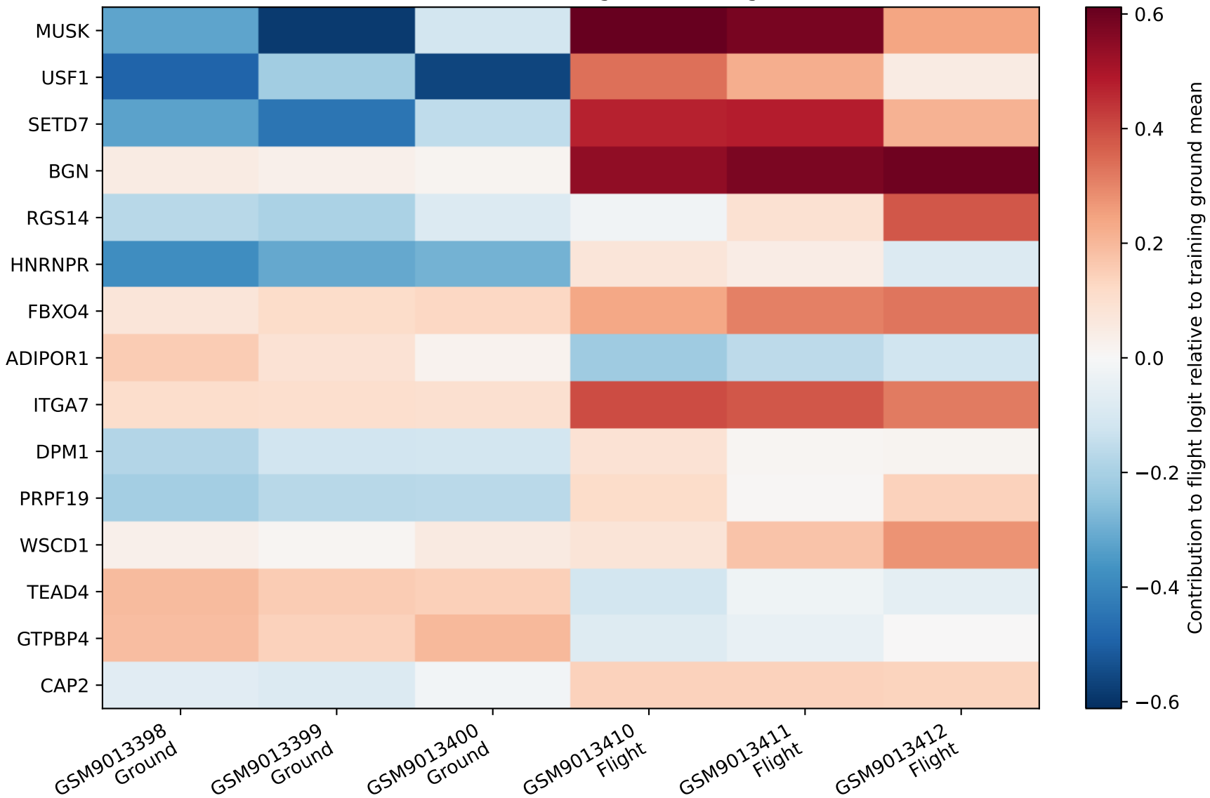
Primary head: genes supporting individual held-out OS chips Positive contribution raises the flight score; negative lowers it
