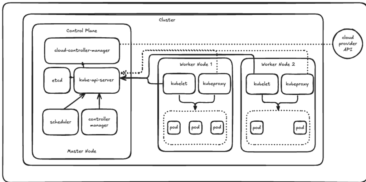
Figure 2-2: Typical Kubernetes Architecture
