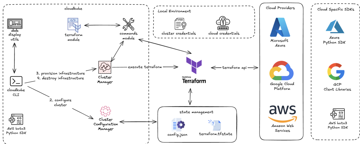
Figure 4-1: cloudkube architecture diagram
