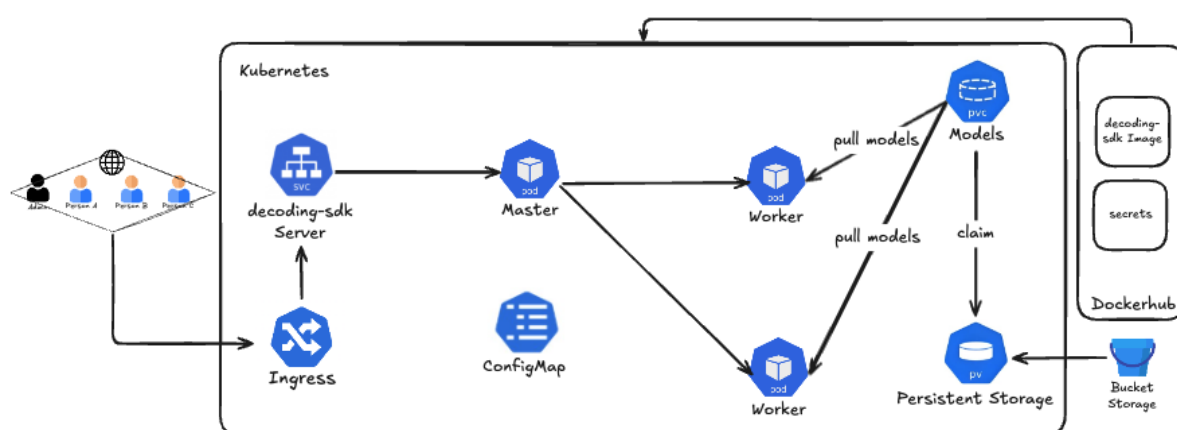
Figure 3-1: Architecture Diagram for SpeechLab ASR Application
