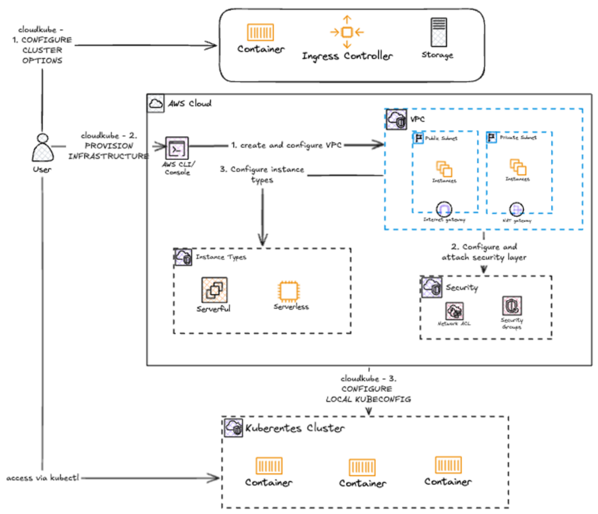
Figure 3-2: Workflow for creating a Kubernetes cluster with cloudkube
