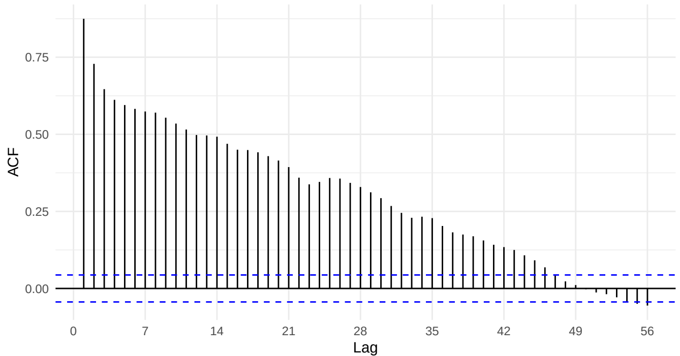
ACF -- daily load (training set)
