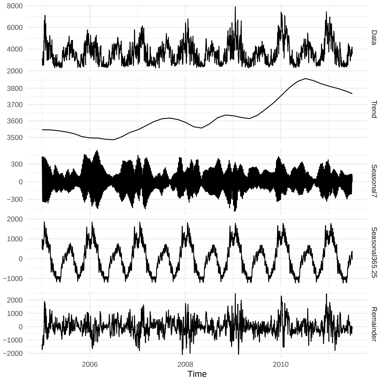
MSTL decomposition of daily load
