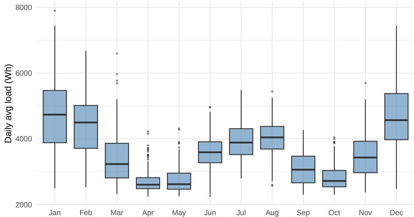
Annual seasonal pattern: load by month
