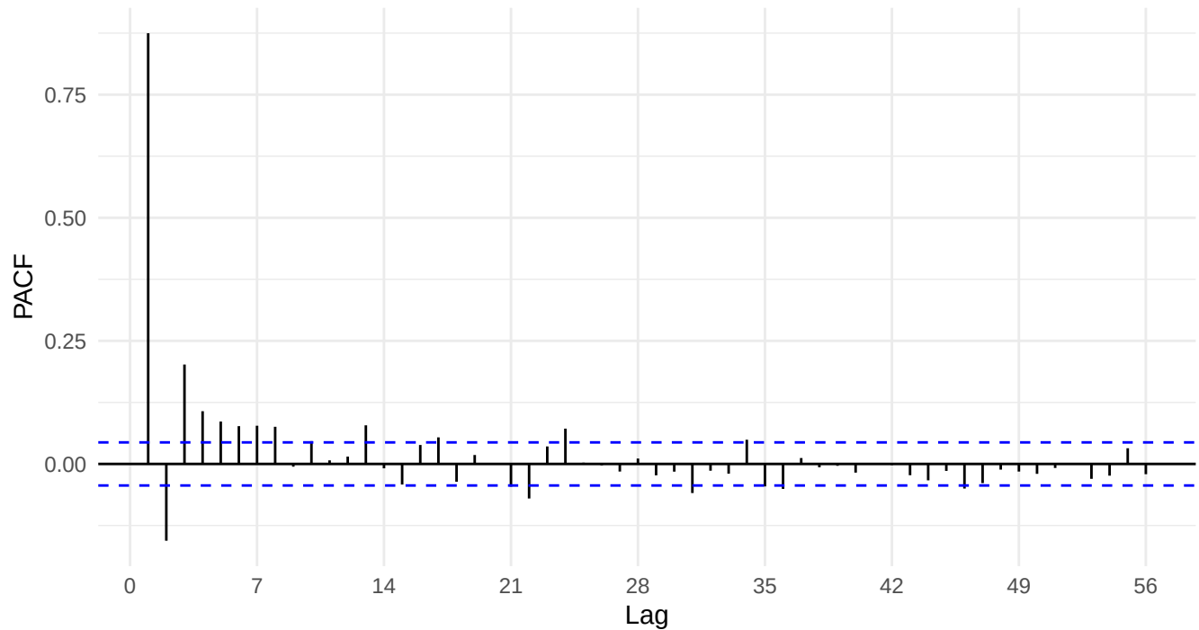
PACF -- daily load (training set)
