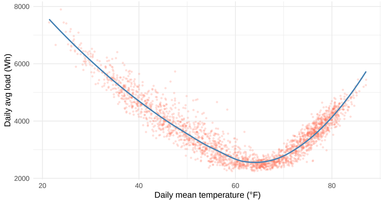
Load vs. temperature
