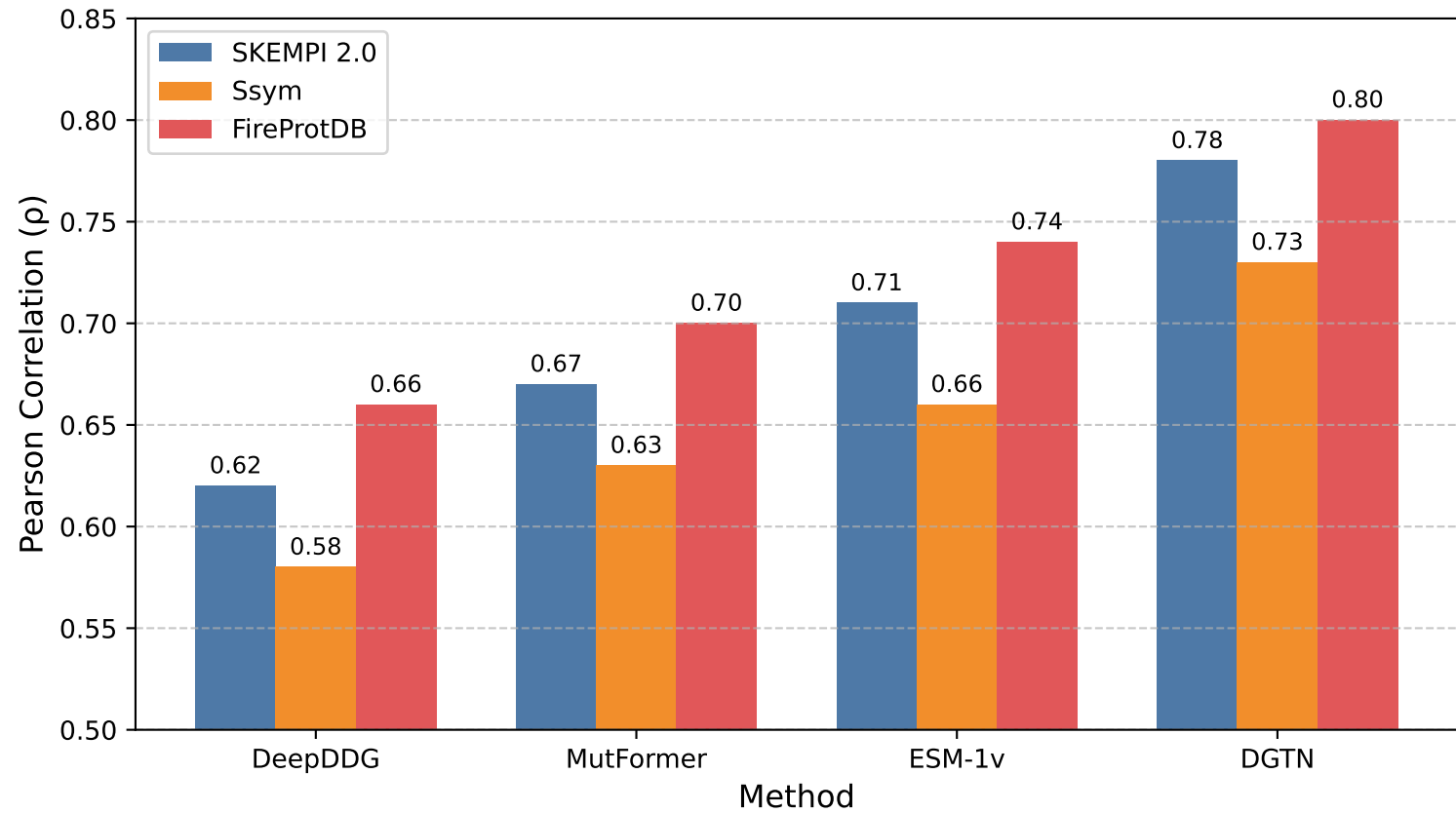
Cross-Dataset Generalization (Trained on ProTherm)
