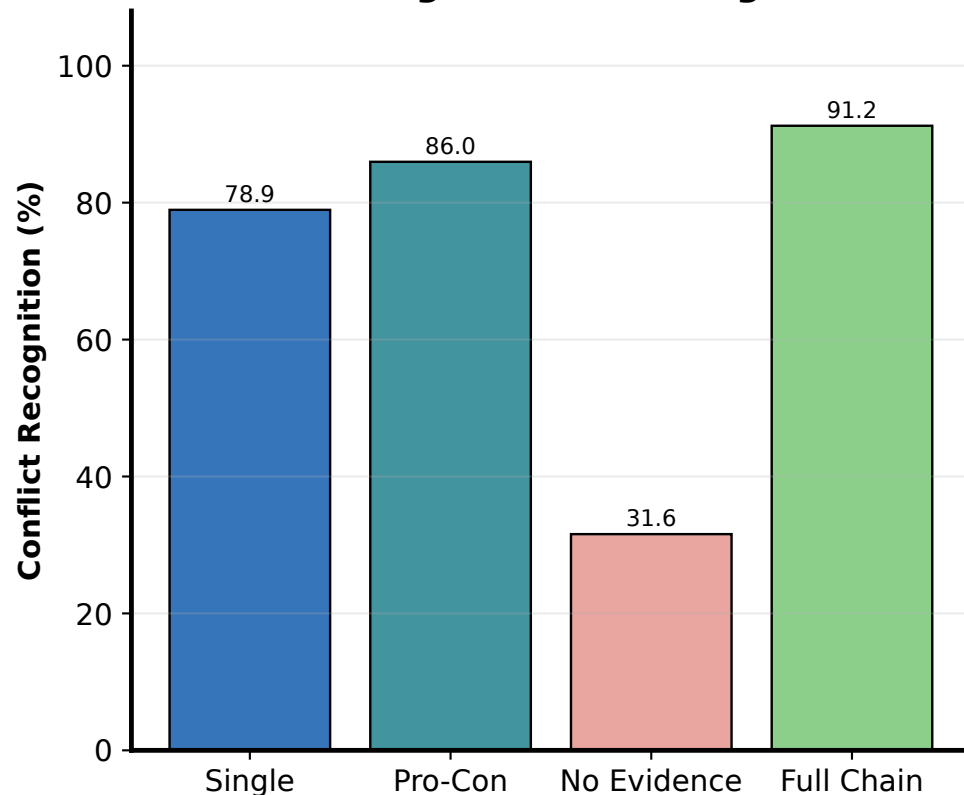
Conflict Recognition across Agent Links
