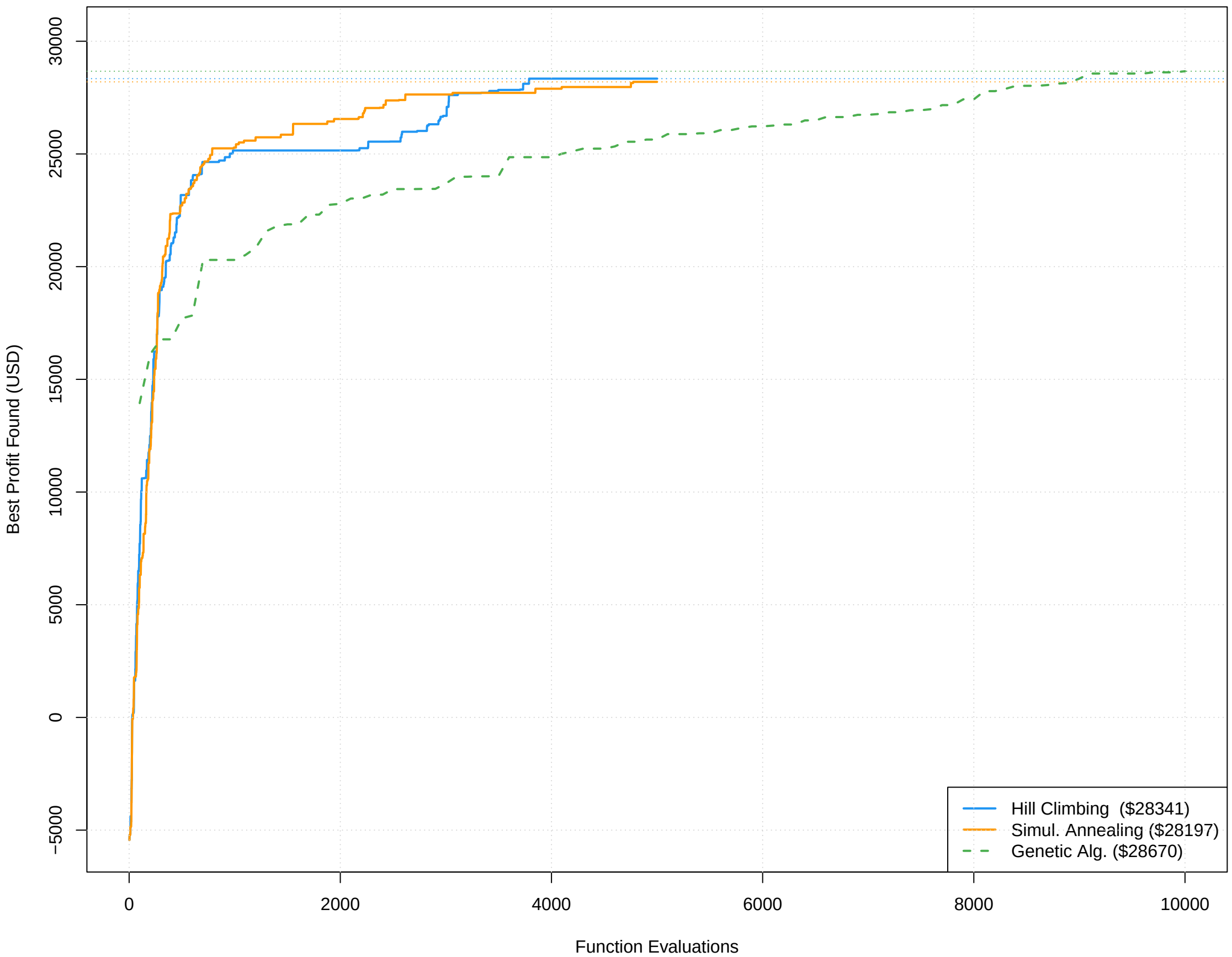
Convergence Comparison – Week 20 (O1)
