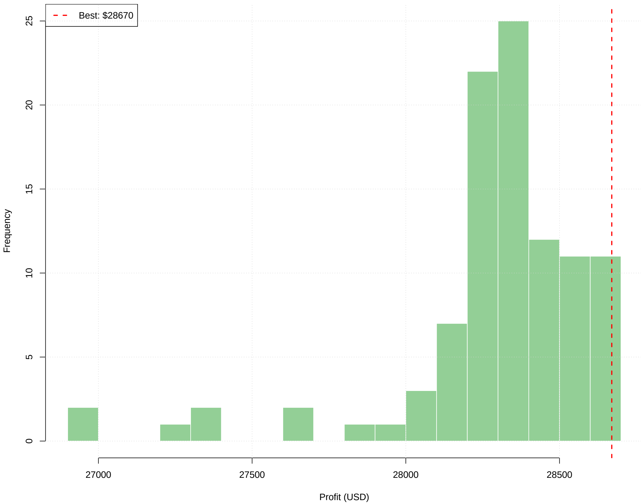
GA Final Population – Fitness Distribution Week 20 (O1)
