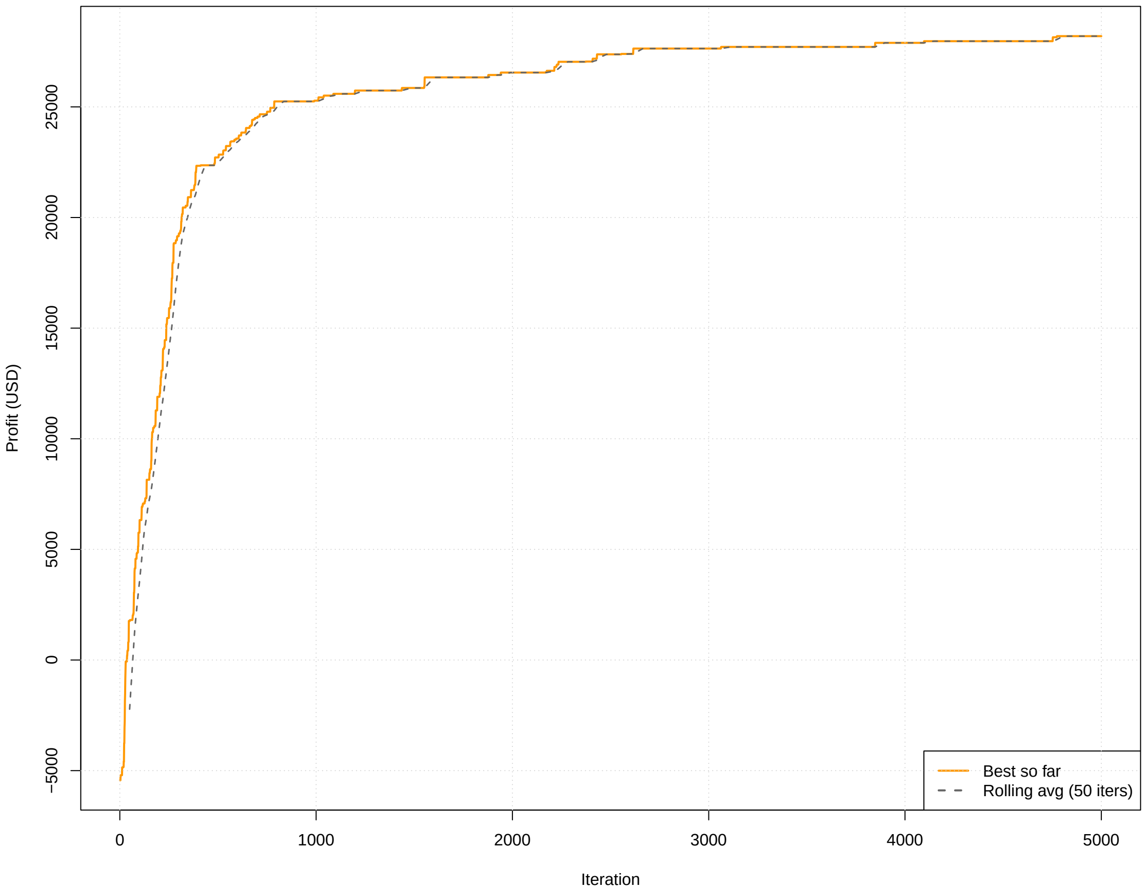
SANN – Best-so-far vs Rolling Average
