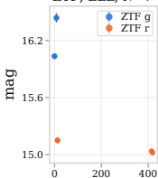
ZTF, ELL, N=7
