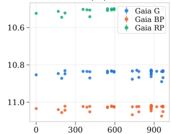
9. ZTF, E, n=62
