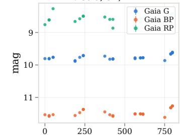
7. Gaia, SR, n=72
