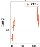
ZTF, M, N=22
