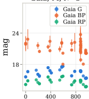
Gaia, M, N=12
