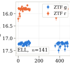
ZTF mag (observed)
