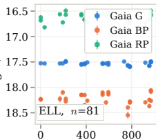
Gaia mag (observed)
