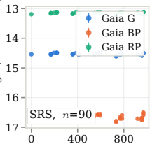
Gaia mag (observed)
