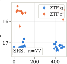
ZTF mag (observed)
