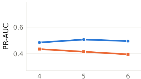
Logistic regression
