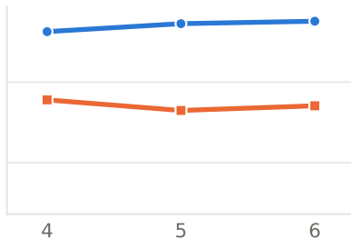
Random forest
