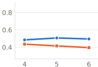
Logistic regression
