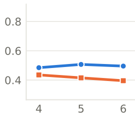
Logistic regression
