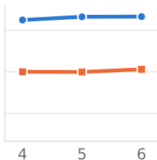
LightGBM
