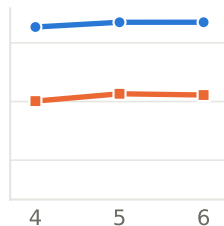
XGBoost
