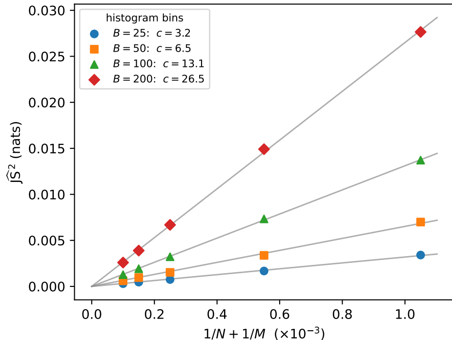
(b) \widehat{JS}^2 is linear in 1/N + 1/M with slope \propto B
