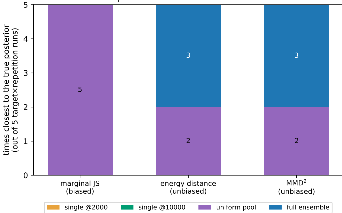
Which sampler is closest to the NUTS reference? The answer flips between the biased and the unbiased metrics
