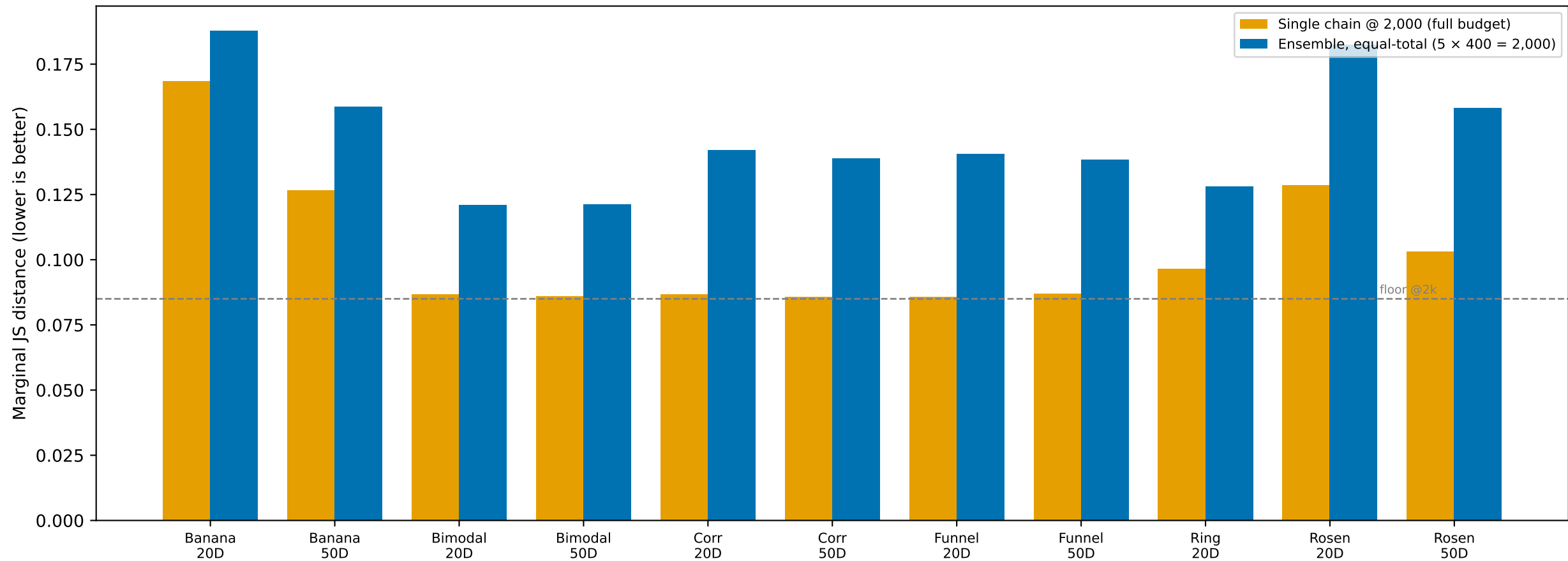
Under an equal total budget of 2,000 samples, the ensemble is worse on every configuration
