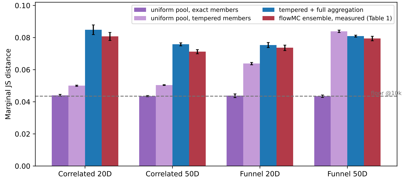
Exact tempered members + the aggregation stack reproduce the measured flowMC ensemble
