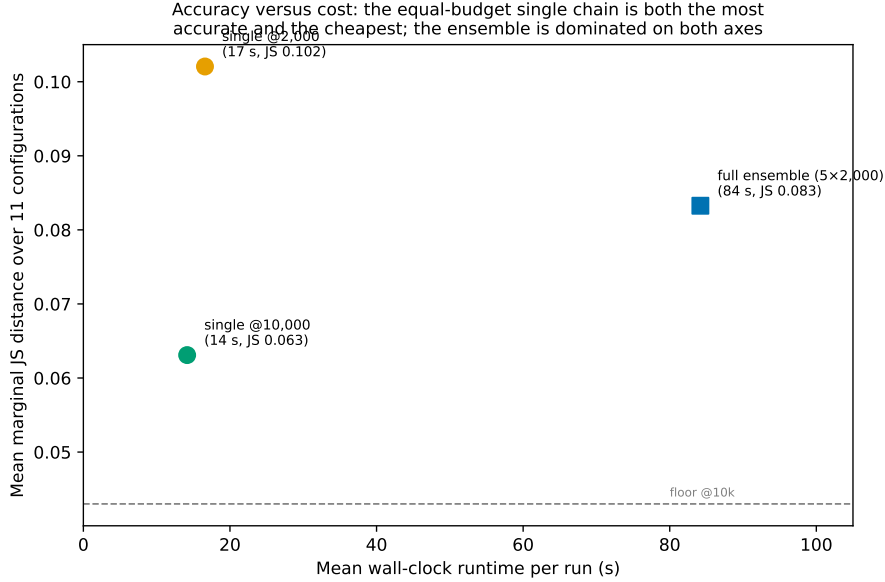
Figure 12: Accuracy versus cost (mean over the eleven configurations; measured wall-clock run-times). The equal-budget single chain is simultaneously the most accurate and the cheapest option, so the ensemble is dominated on both axes: it costs about six times more and is less accurate.
