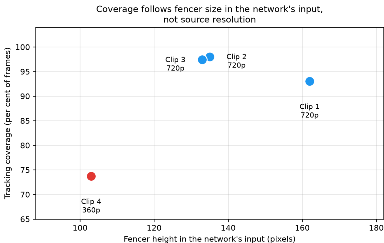
Figure 4.4: Coverage against fencer height in the network's input. Source resolution is annotated. Clip 4 is both the smallest fencer and the lowest coverage, while the 720p clips at similar fencer heights reach similar coverage.
