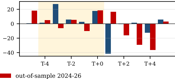
A: drift-signed bond-minus-stock (bp/day)
