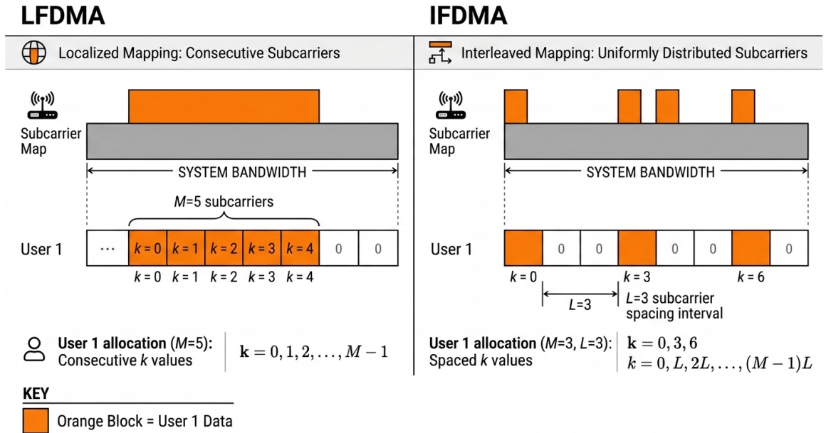
Figure 2.7 Localized and interleaved SC-FDMA subcarrier allocation
