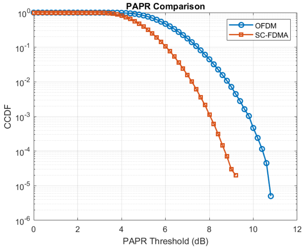
Figure 3.3 CCDF comparison of OFDM and SC-FDMA PAPR
