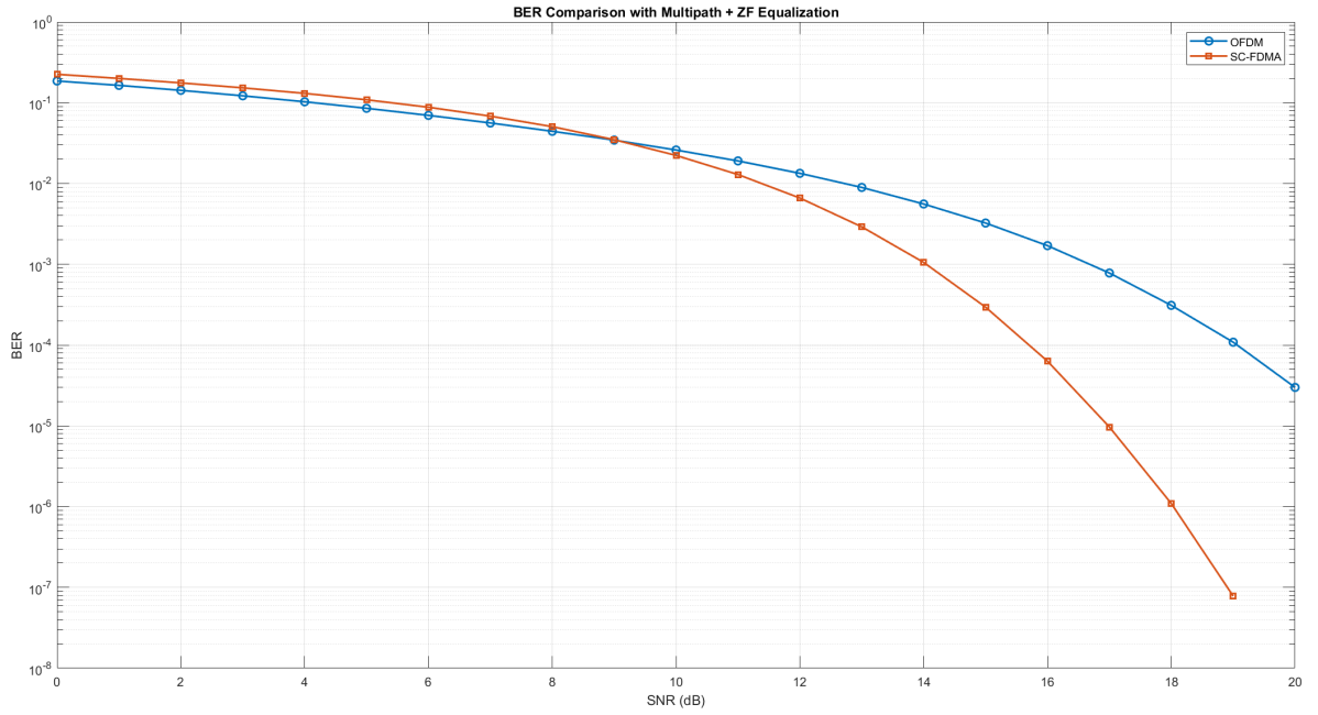
Figure 3.2 BER performance comparison between OFDM and SC-FDMA
