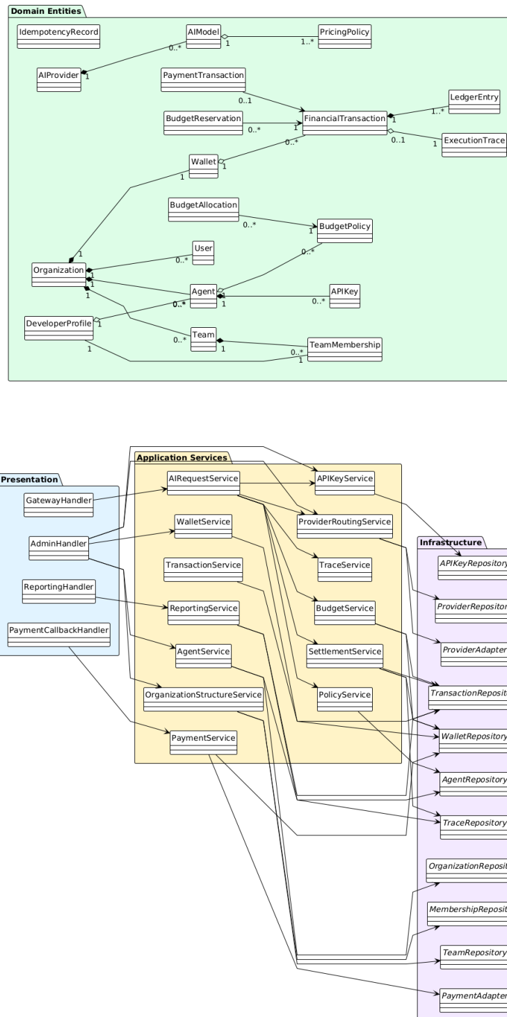
Design Class Diagram Overview - Asymptotic
