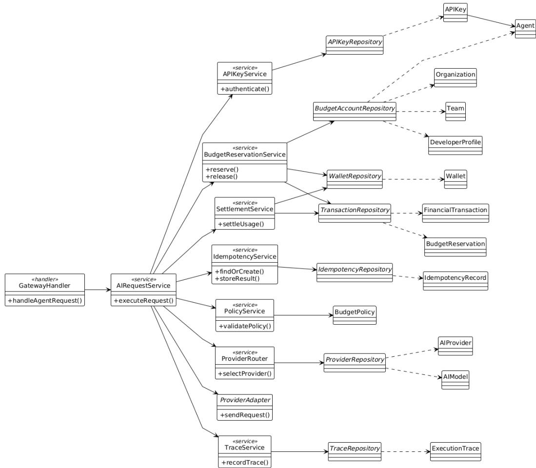
Design Class Diagram - Gateway Request Flow
