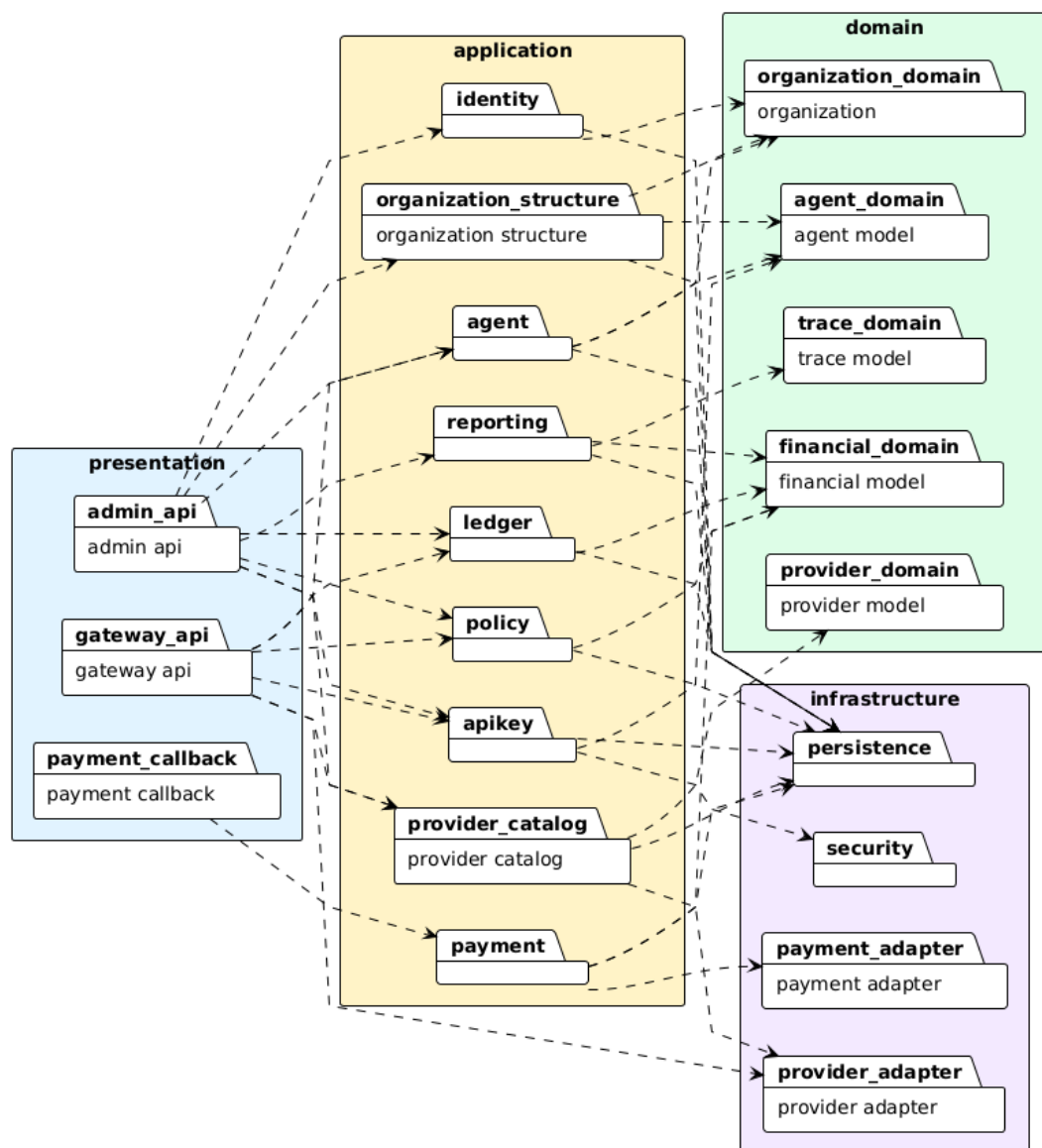
Package Diagram - Asymptotic AI Agent Financial Gateway
