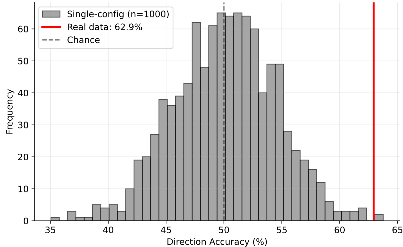
Single-Config Permutation Test (2 / 1000 \geq real, p = 0.00300 )
