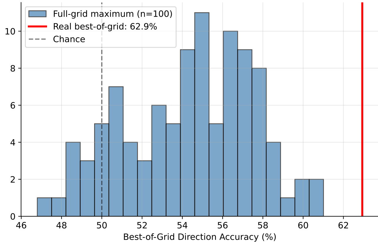
Full-Grid Permutation Test (0 / 100 \geq real, p = 0.0099 )
