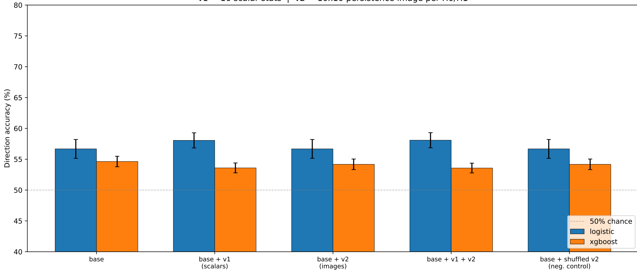
V12: TDA Representation Ablation (leak-safe per-fold imager fit) v1 = 16 scalar stats | v2 = 10x10 persistence image per H0/H1
