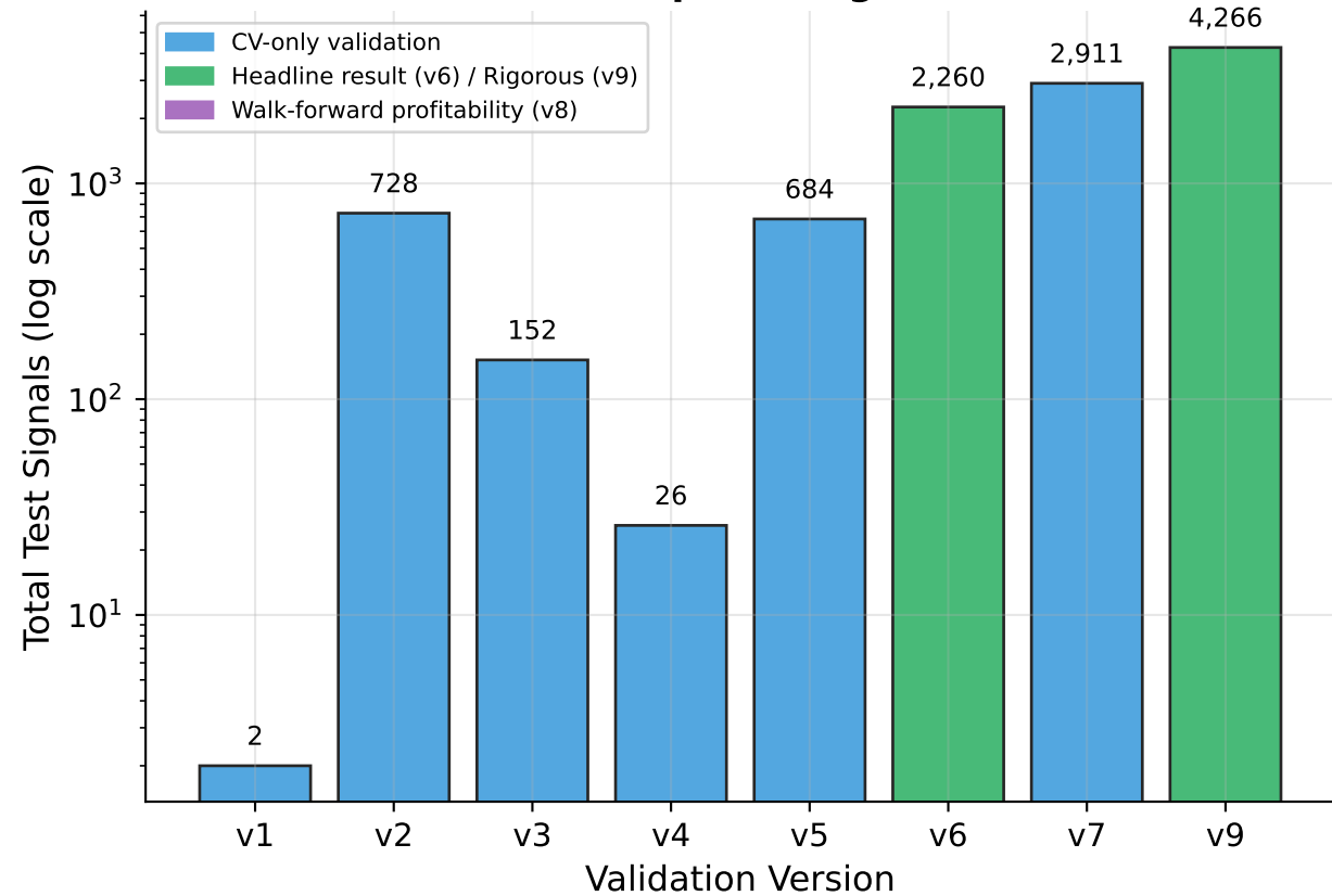
Sample Size Progression (more samples → tighter CI)
