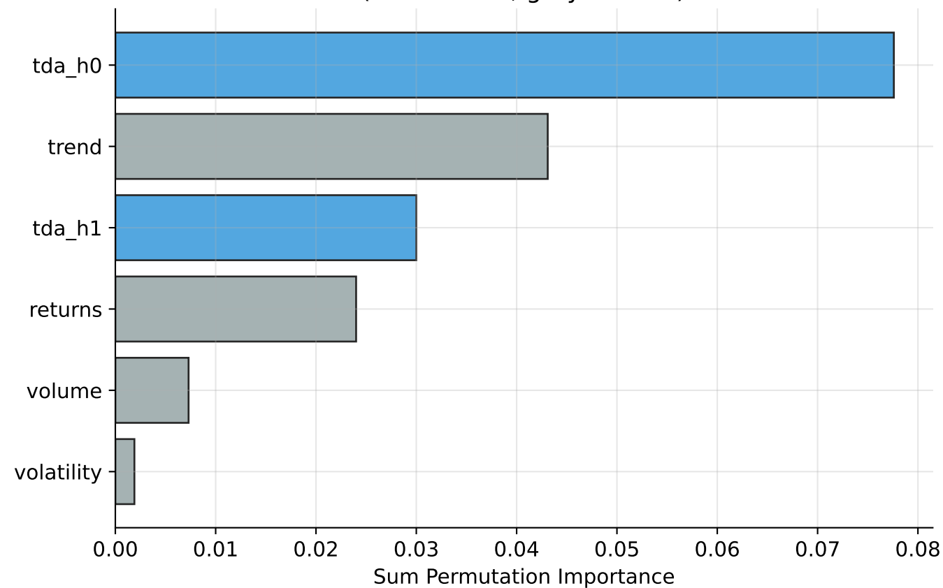
Grouped Feature Importance (blue = TDA, gray = base)
