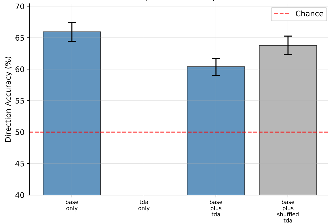
Ablation: Does TDA Help? (Wilson 95% CI)
