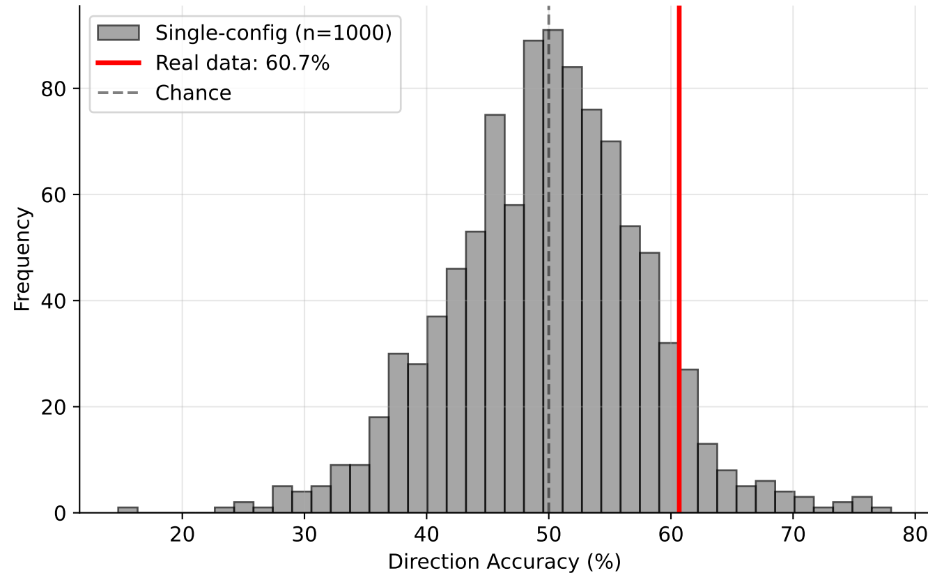
Single-Config Permutation Test (73 / 1000 \geq real, p = 0.07393 )
