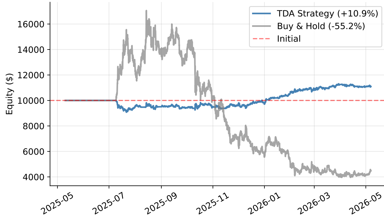
ADA — coinbase_taker (38 trades, Sharpe 0.88)
