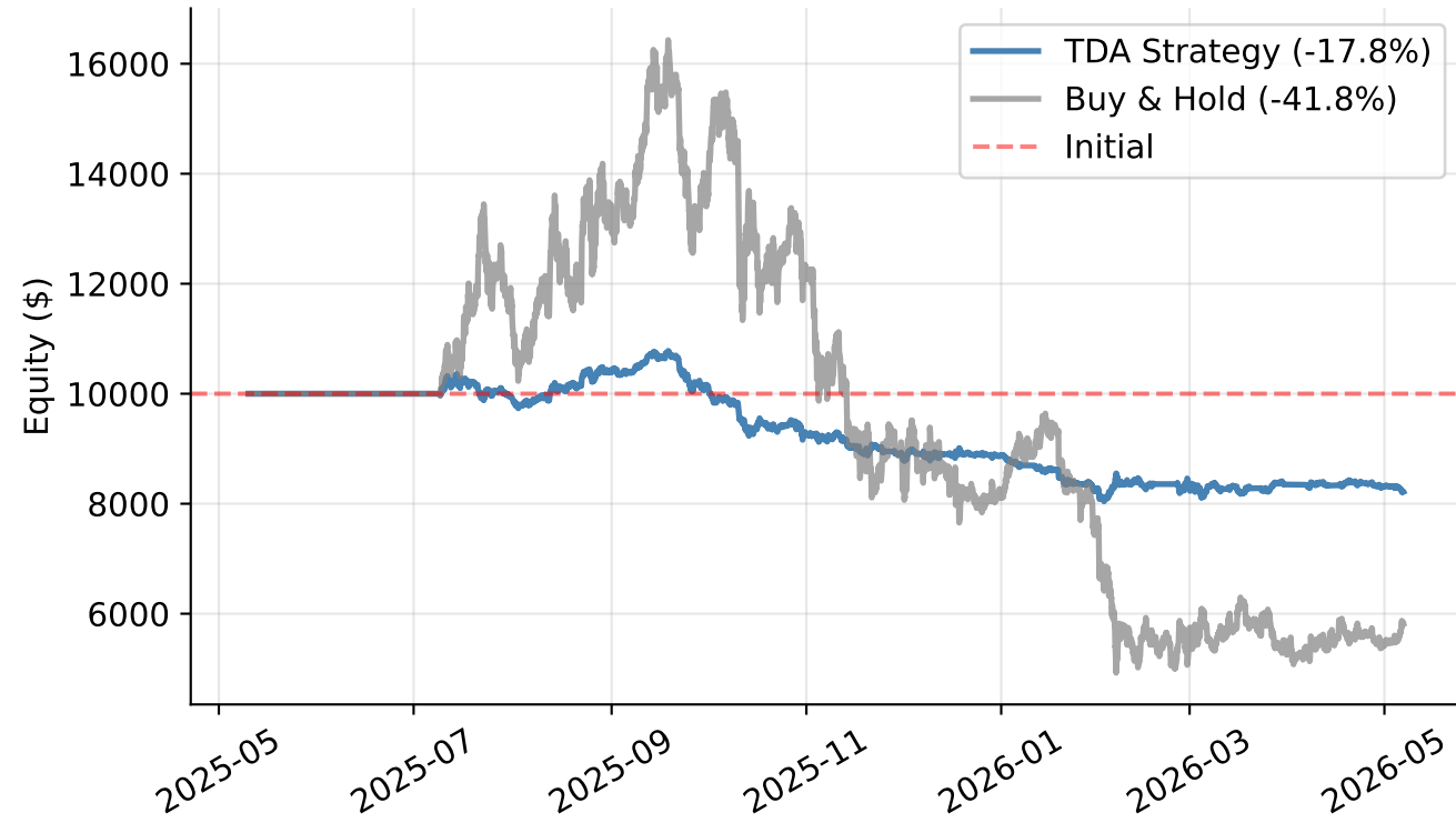
SOL — coinbase_taker (37 trades, Sharpe -1.63)
