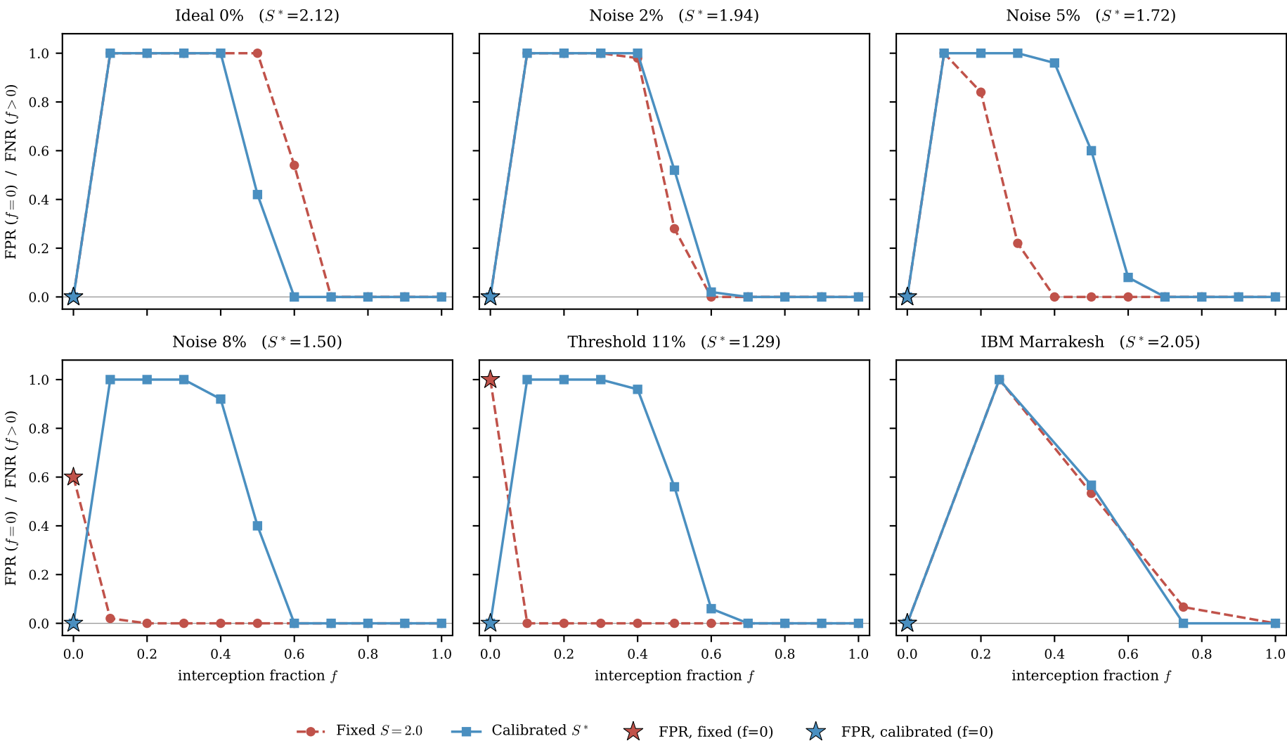
E91 detection error across the full attack sweep: fixed vs. noise-calibrated CHSH threshold
