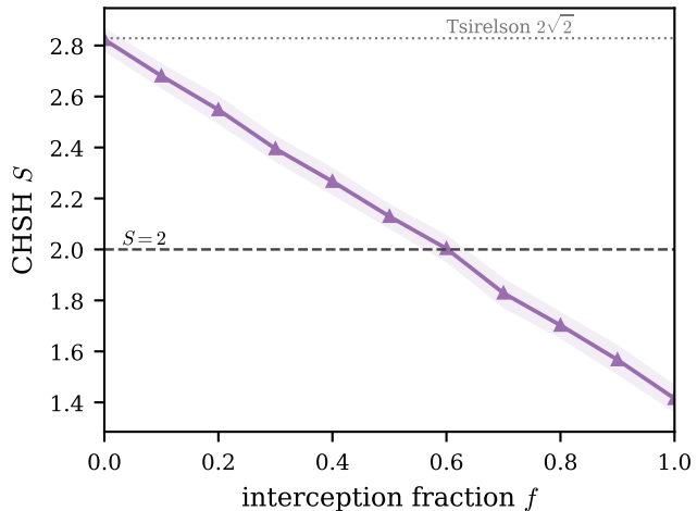
(b) CHSH S vs attack fraction (E91)
