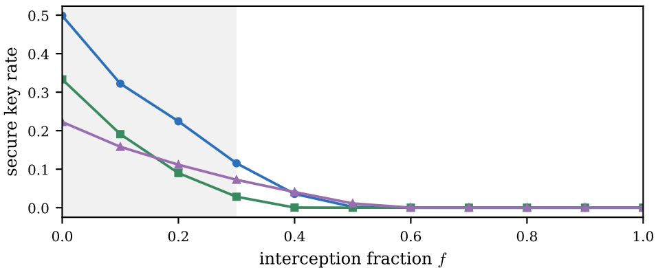
(b) secure key rate vs attack fraction
