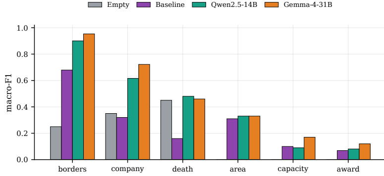
Figure 3: Per-relation validation macro-F1: empty baseline, official baseline, Qwen2.5-14B, and Gemma-4-31B. Gemma-4-31B beats the official baseline on all six relations.
