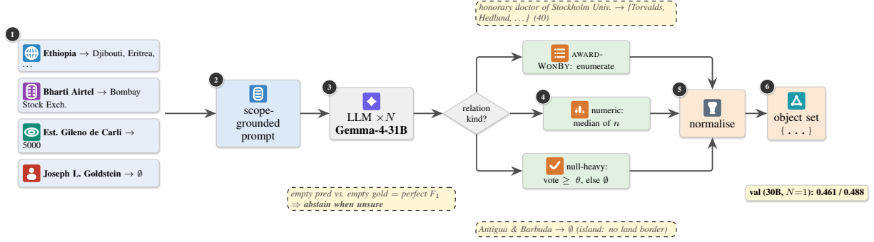
Figure 1: System pipeline (no trainable parameters). Real dataset instances (left, stage 1), shown with entity-type icons and their gold objects, are each rendered into a scope-grounded chat prompt (stage 2); the model is sampled N times (stage 3, cached), and the samples are aggregated by relation kind (stage 4): median for numeric relations, consistency voting with abstention (keep an object only if it appears in \geq \theta of samples, else \emptyset ) for the null-heavy string relations, and enumeration for AWARDWONBY; a final normalisation matches the evaluator exactly. Dashed callouts give worked examples of the abstention cases. The reported Gemma-4-31B score uses a single sample ( N=1 , voting off); the N -sample voting path is exercised by the 14B ablation (Section 7).
