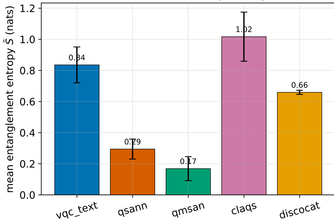
(a) the trained circuits carry entanglement
