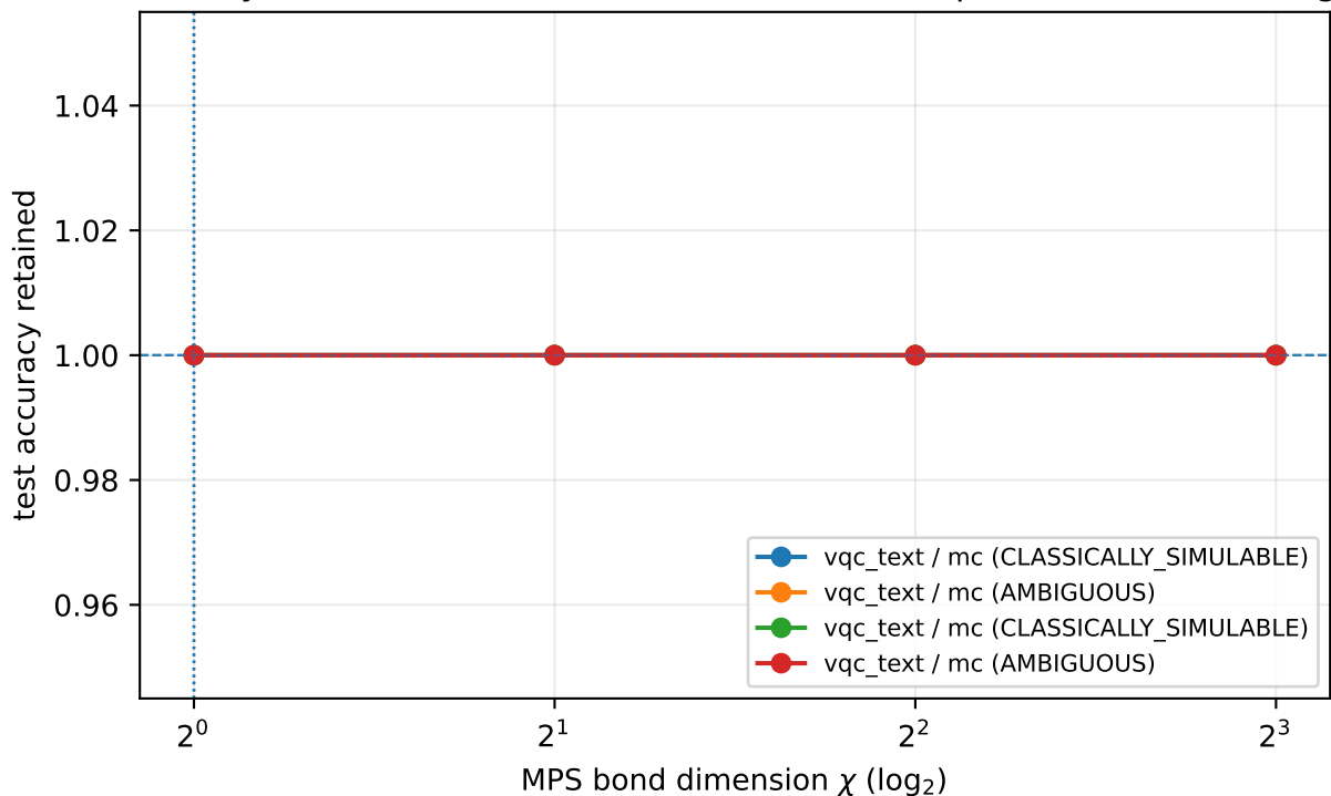
Accuracy retained vs bond dimension (was the quantum load-bearing?)
