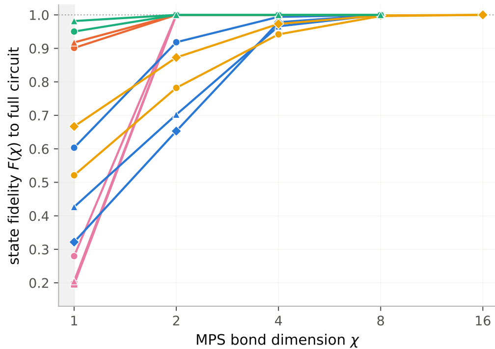
(b) state fidelity climbs with \chi
