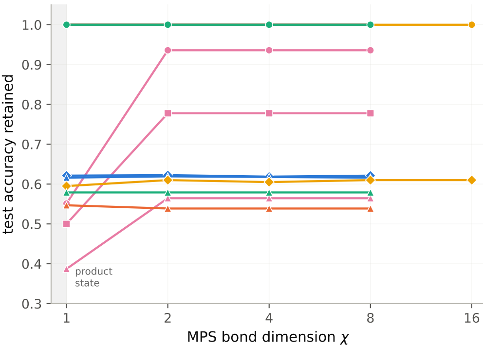
(a) predictions recovered at \chi = 1
